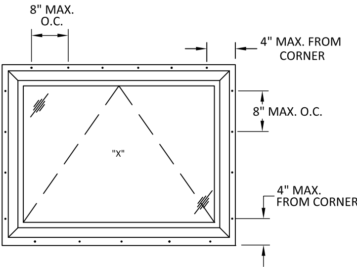
TYPICAL ANCHOR LAYOUT NAIL FIN INSTALLATION
