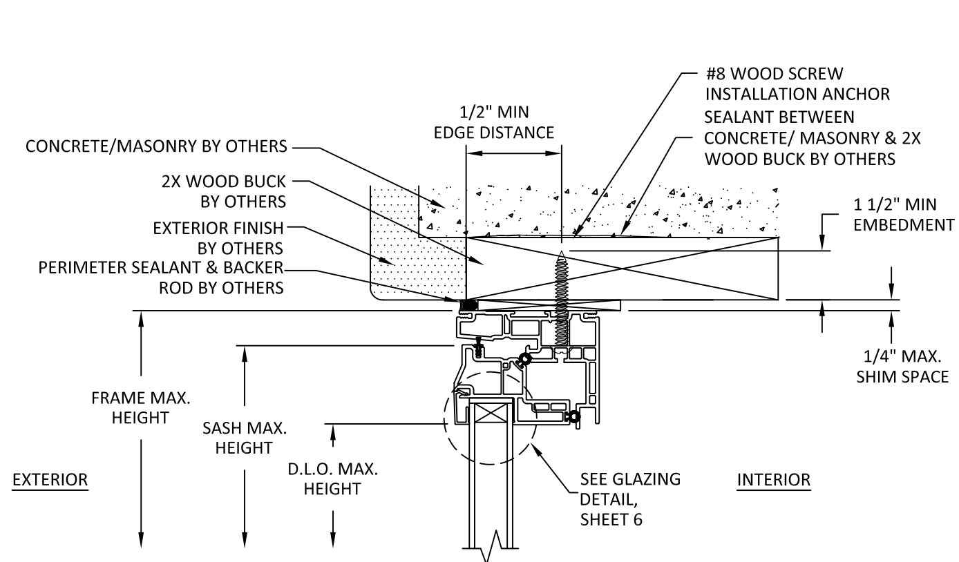
A 4 VERTICAL SECTION THROUGH FRAME INSTALLATION WOOD SUBSTRATE
