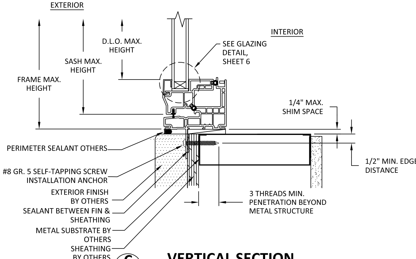
C 3 VERTICAL SECTION NAIL FIN INSTALLATION METAL SUBSTRATE
