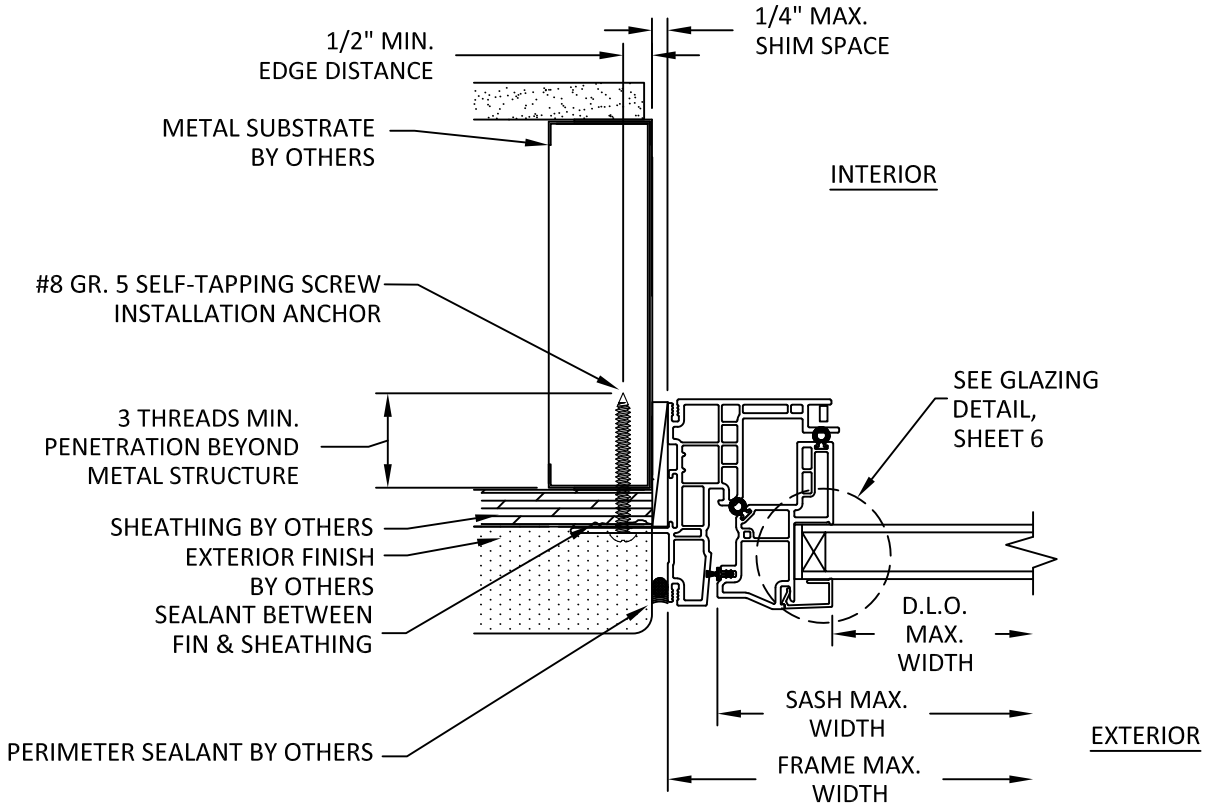
B 3 HORIZONTAL SECTION NAIL FIN INSTALLATION METAL SUBSTRATE
