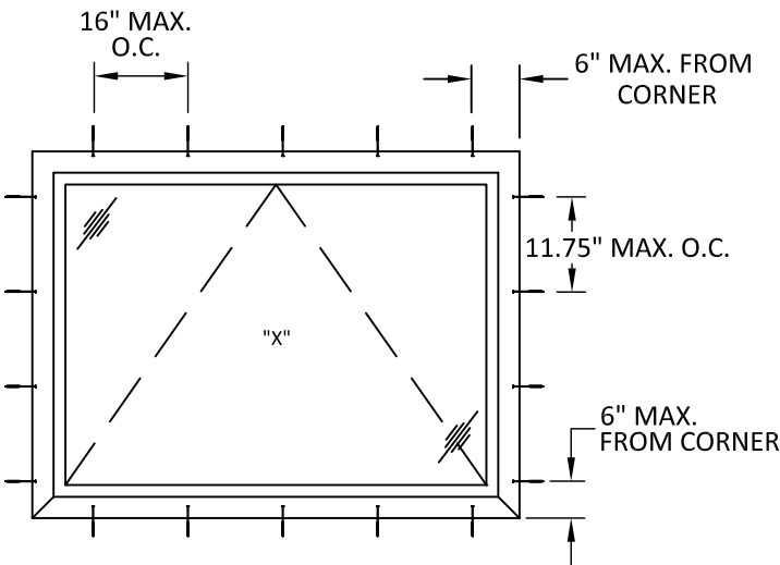
TYPICAL ANCHOR LAYOUT CLIP OR THROUGH FRAME INSTALLATION
