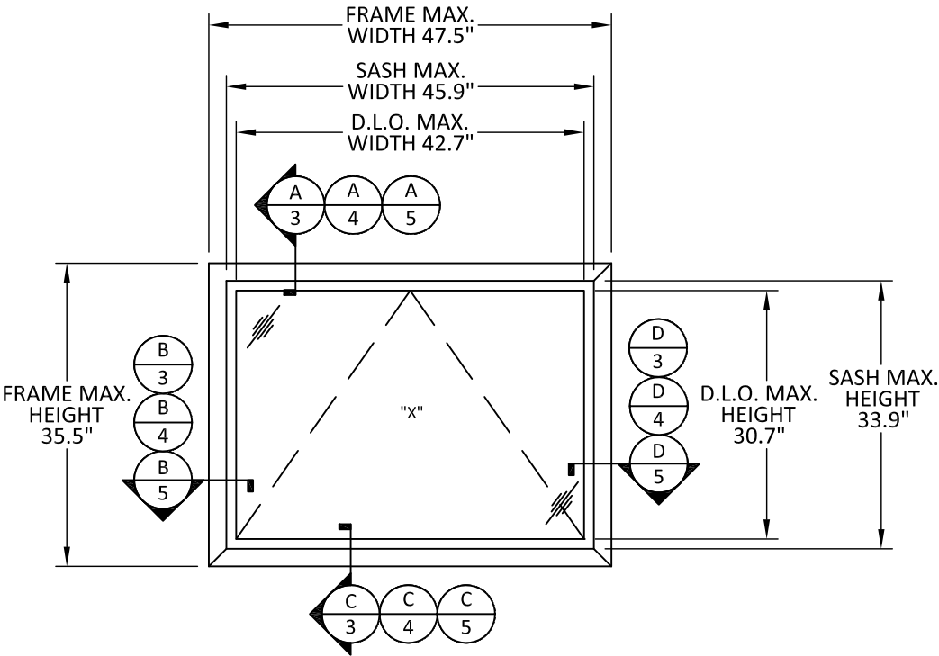
TYPICAL ELEVATION AWNING WINDOW
