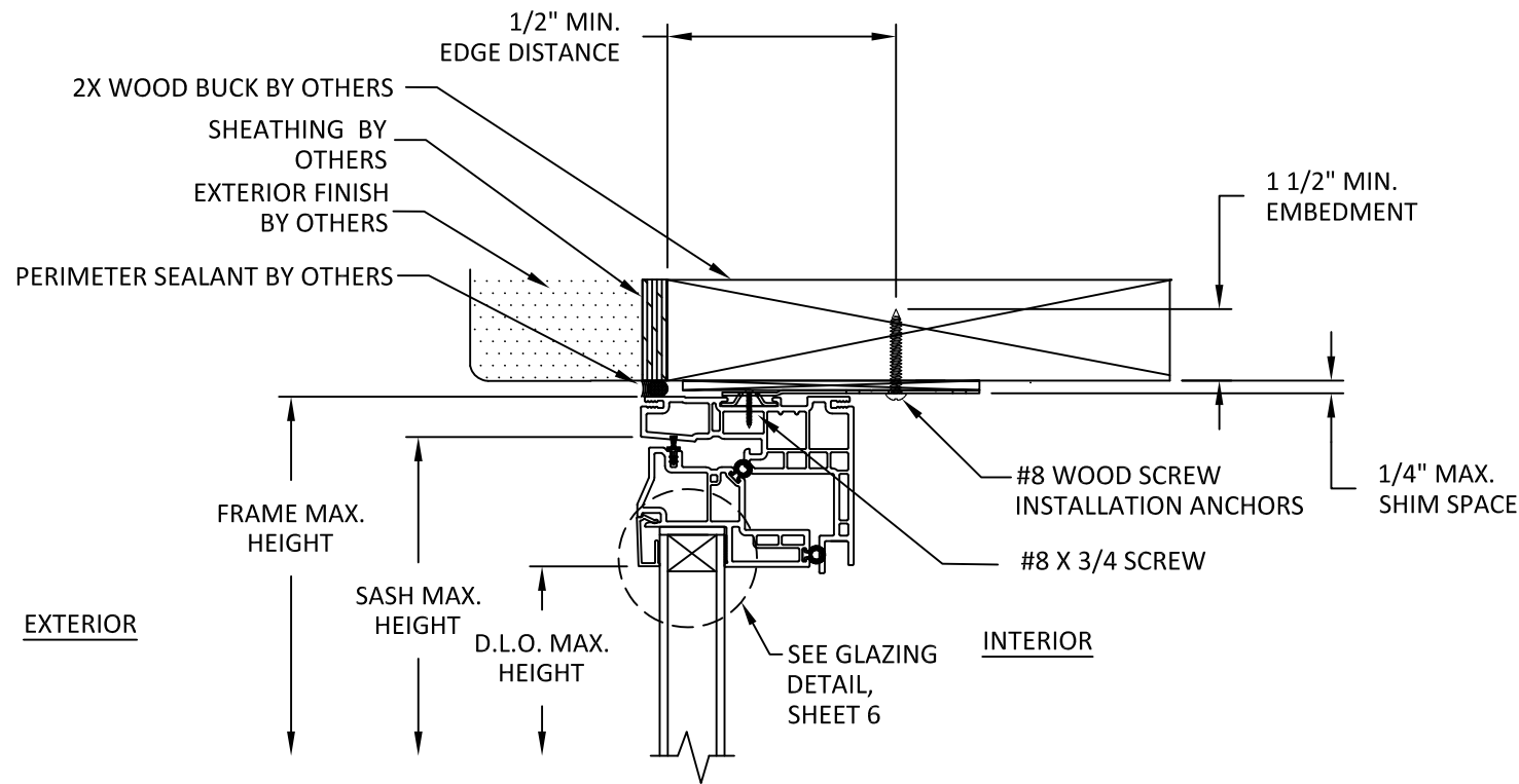
A 5 VERTICAL SECTION CLIP INSTALLATION WOOD SUBSTRATE
